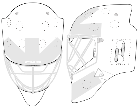
= reinforcements = holes
